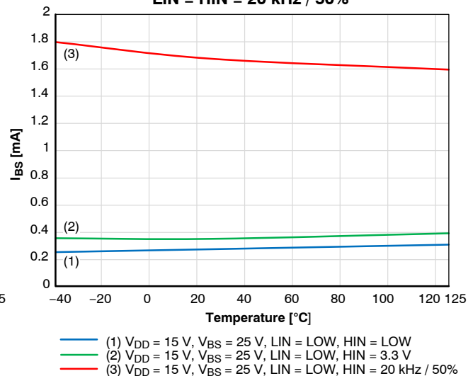
Figure 12. I_{BS} Supply Current V_{BS} = 25\text{ V}
