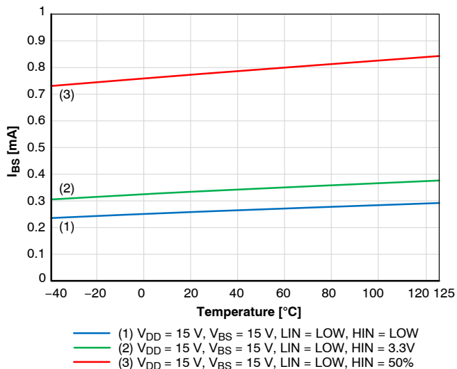
Figure 11. I_{BS} Supply Current V_{BS} = 15\text{ V}
