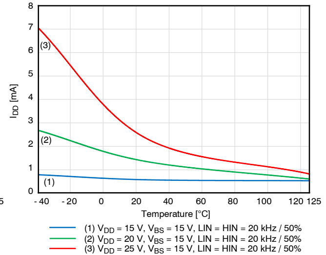
Figure 11. I_{DD} Supply Current V_{DD} = 15\text{--}25\text{ V} , V_{LIN} = \text{HIN} = 20\text{ kHz} / 50\%
