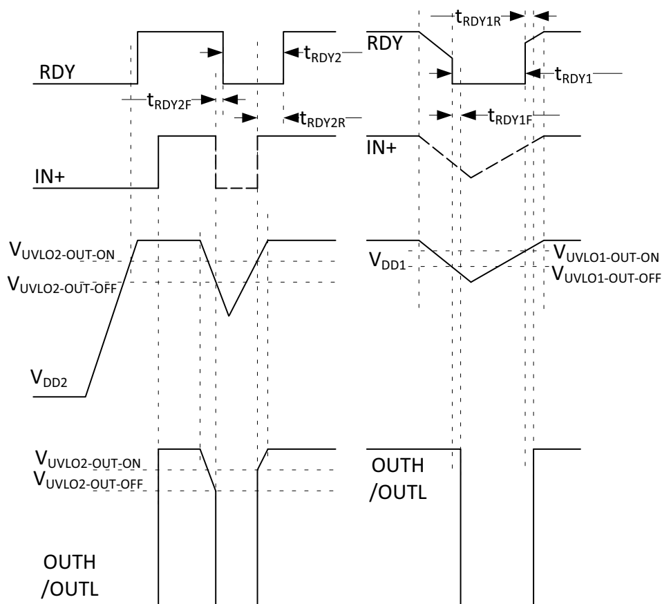
Figure 19. UVLO Diagram
