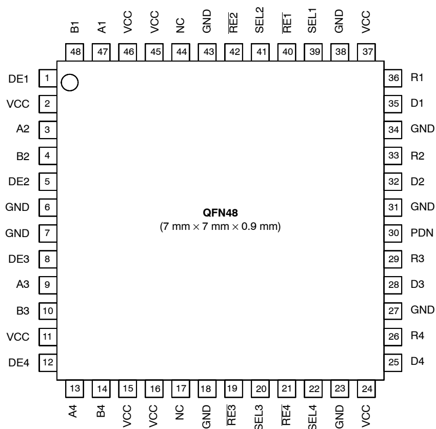
Figure 1. Pinout Diagram (Top View)
