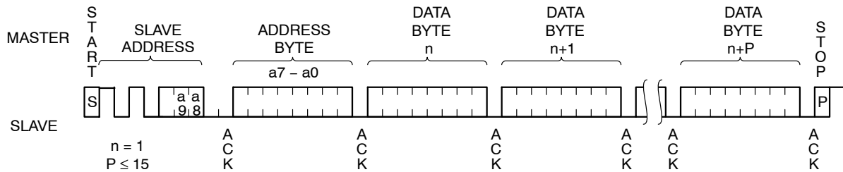
Figure 9. Page Write Sequence
