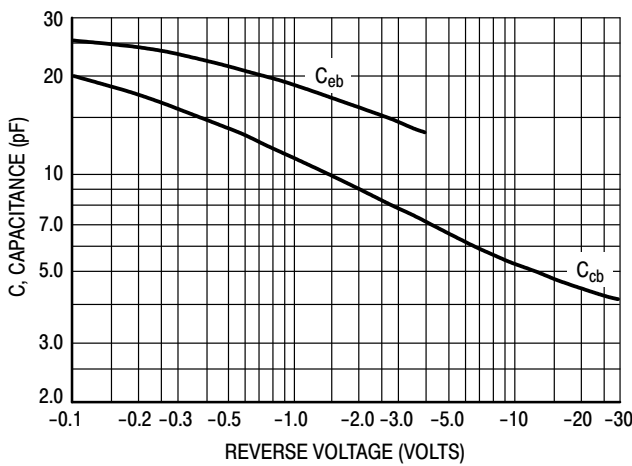
Figure 9. Capacitances
