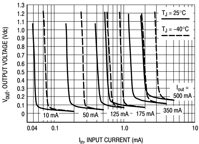
Figure 6. Output Saturation Voltage versus I_{O,OUT}/I_{O,IN}
