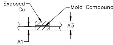
DETAIL "B" Scale 2:1 Side View (Optional)
