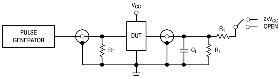
Figure 4. AC Waveforms
