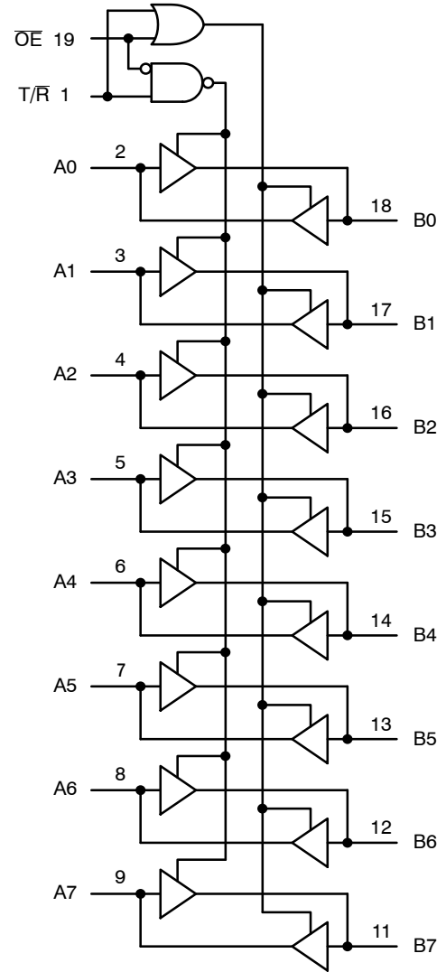
Figure 2. Logic Diagram
