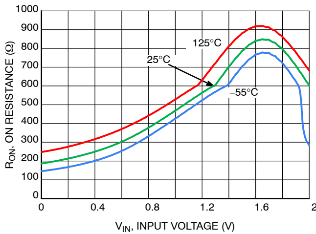
Figure 6. Typical On Resistance V_{CC} = 2\text{ V}
