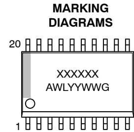
1 SOIC-20W DW SUFFIX CASE 751D
