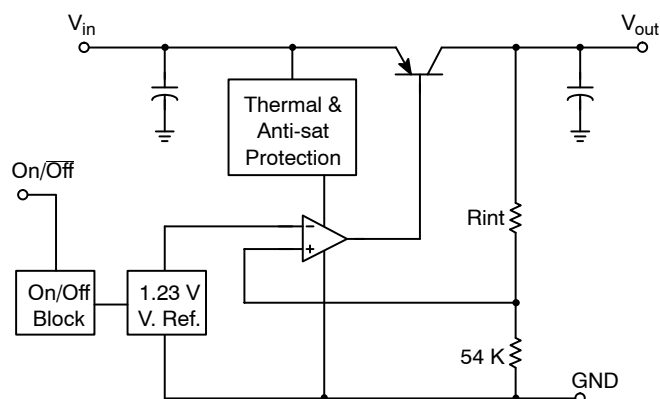
This device contains 41 active transistors
