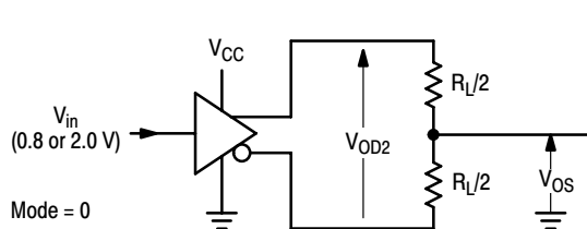
Figure 1. Differential Output Test
