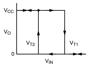
Figure 2. Hysteresis Curve
