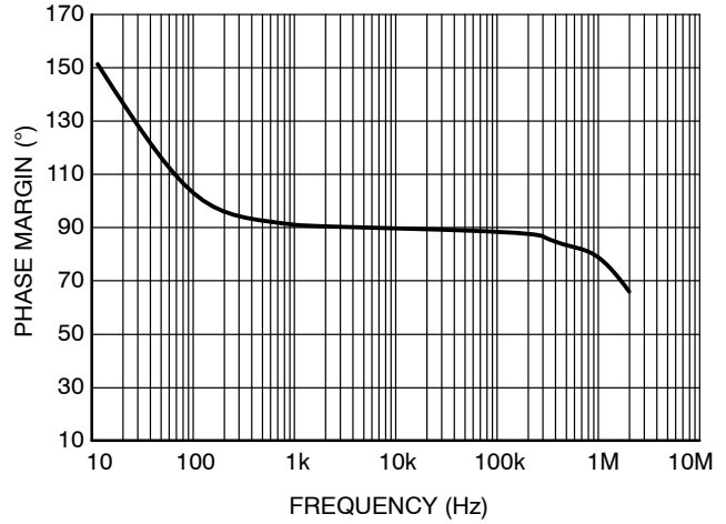
Figure 2. Open Loop Phase Margin ( R_L = 2\text{ k}\Omega , T_A = 25\text{ }^\circ\text{C} , V_S = 5\text{ V} )
