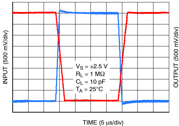
Figure 21. Inverting Large Signal Step Response
