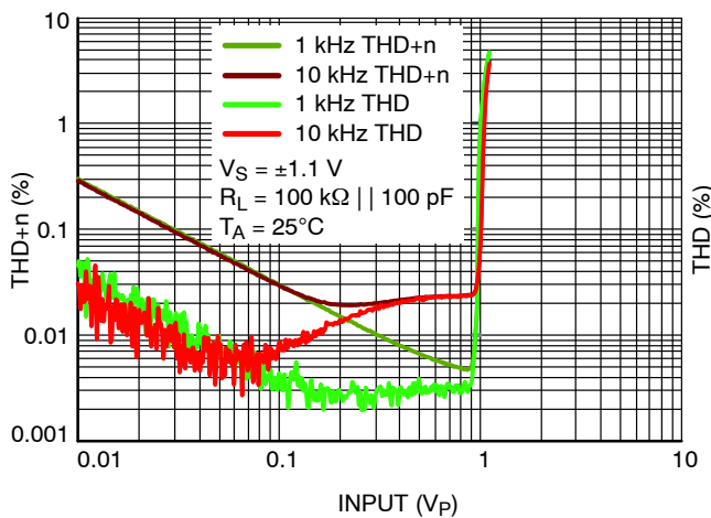
Figure 23. Harmonic Distortion
