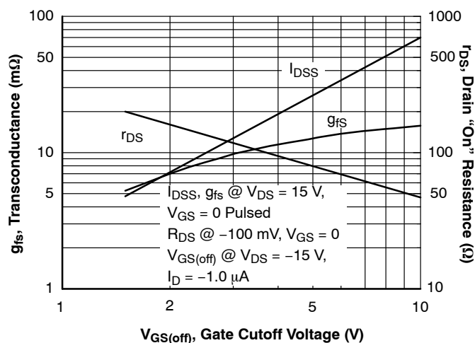
Figure 2. Parameter Interactions
