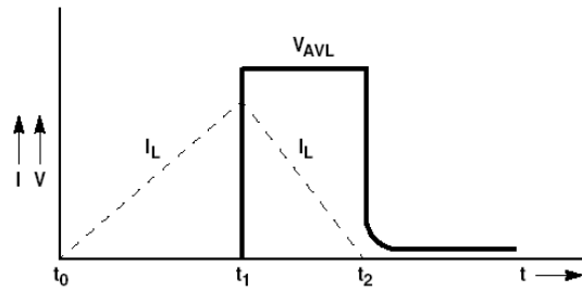
Figure 1. Test Circuit Waveforms
