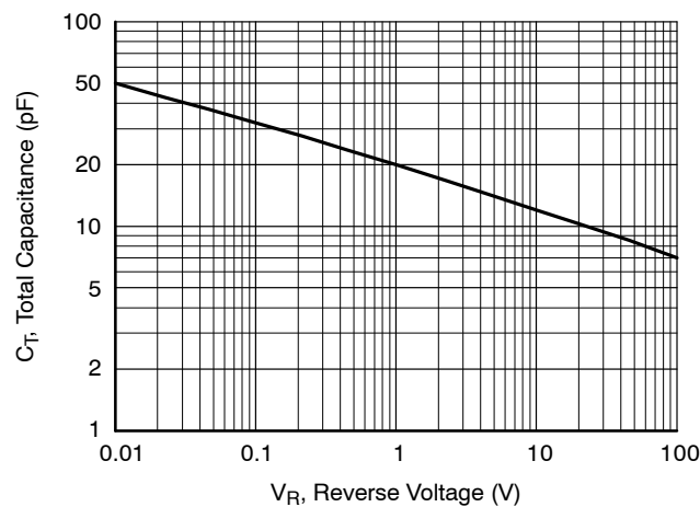
Figure 5. Total Capacitance
