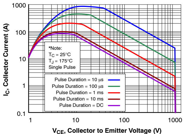
Figure 9. SOA Characteristics
