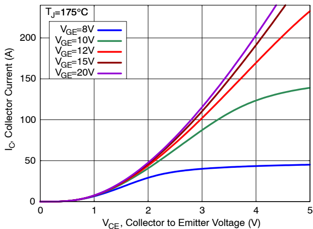
Figure 3. Output Characteristics
