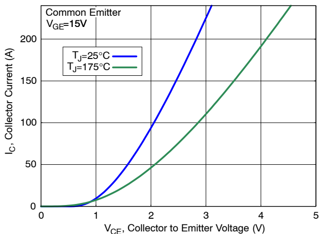
Figure 5. Saturation Characteristics
