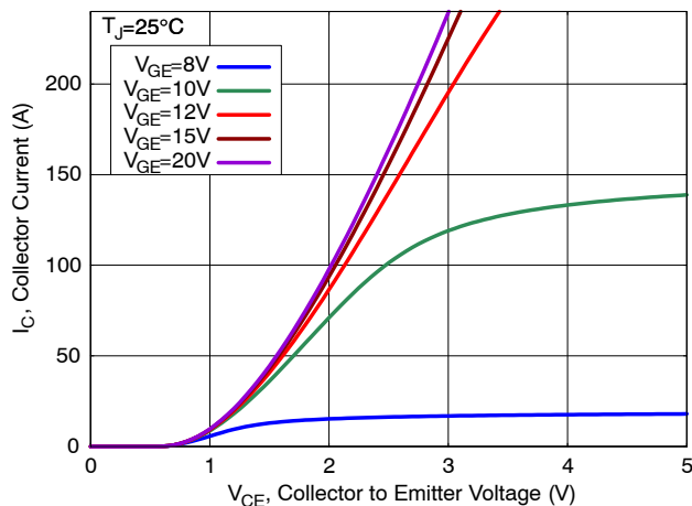
Figure 2. Output Characteristics
