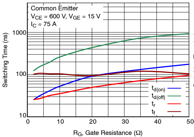
Figure 11. Switching Time vs. Gate Resistance (T J = 175°C)
