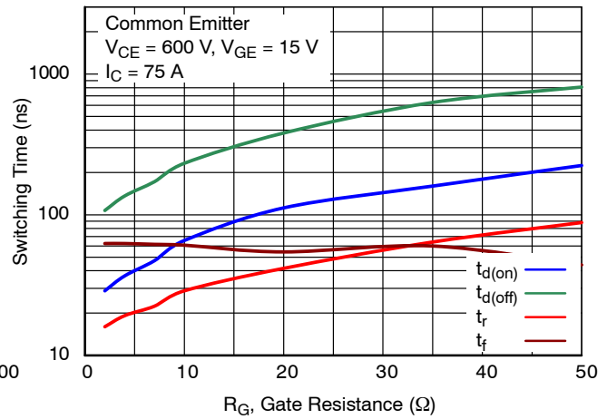
Figure 10. Switching Time vs. Gate Resistance (T J = 25°C)
