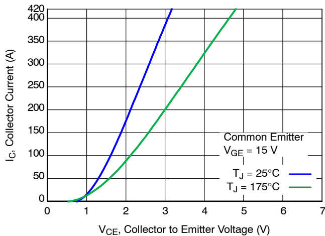
Figure 5. Saturation Characteristics
