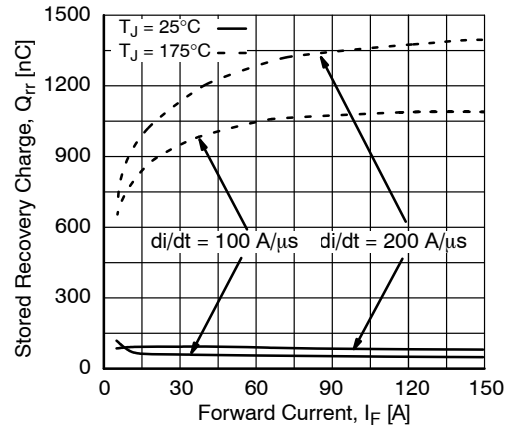
Figure 20. Stored Charge
