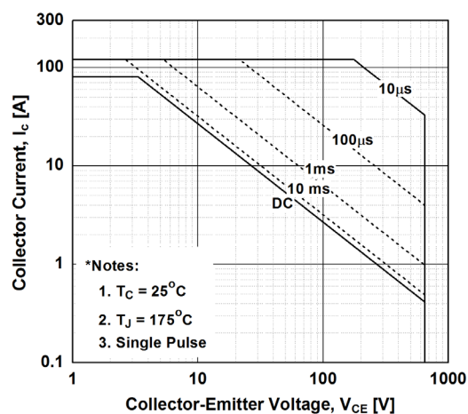
Figure 16. SOA Characteristics
