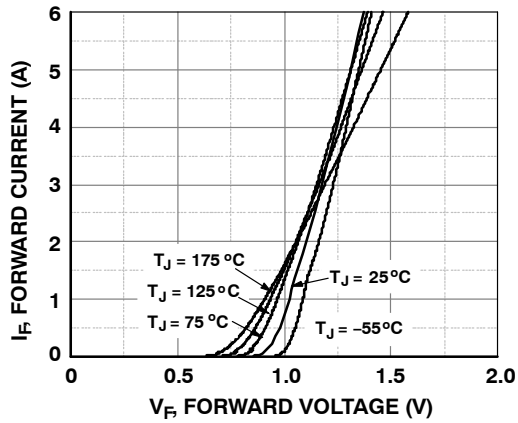
Figure 1. Forward Characteristics
