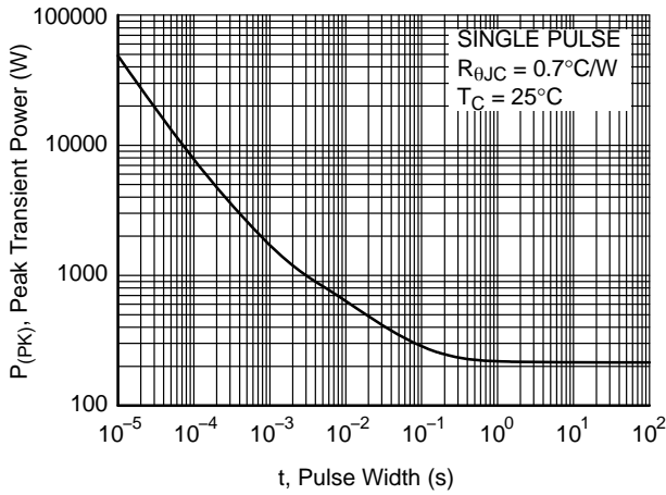
Figure 13. Single Pulse Maximum Power Dissipation for FDP2D3N10C
