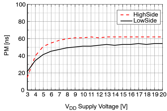
Figure 34. Output Pulse-Width Matching vs. V_{DD} Supply Voltage
