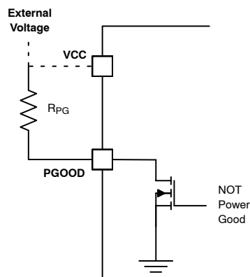
Figure 44. PGOOD Block Diagram
