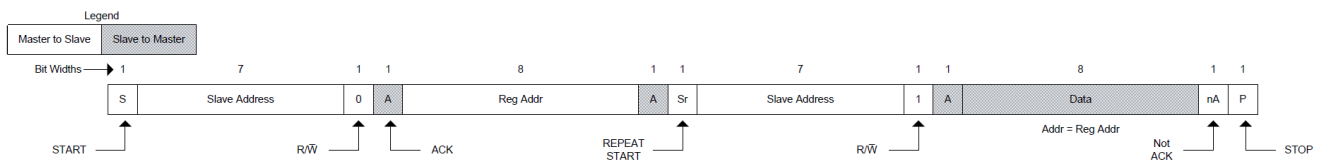
Figure 35. Single Register Read Transaction
