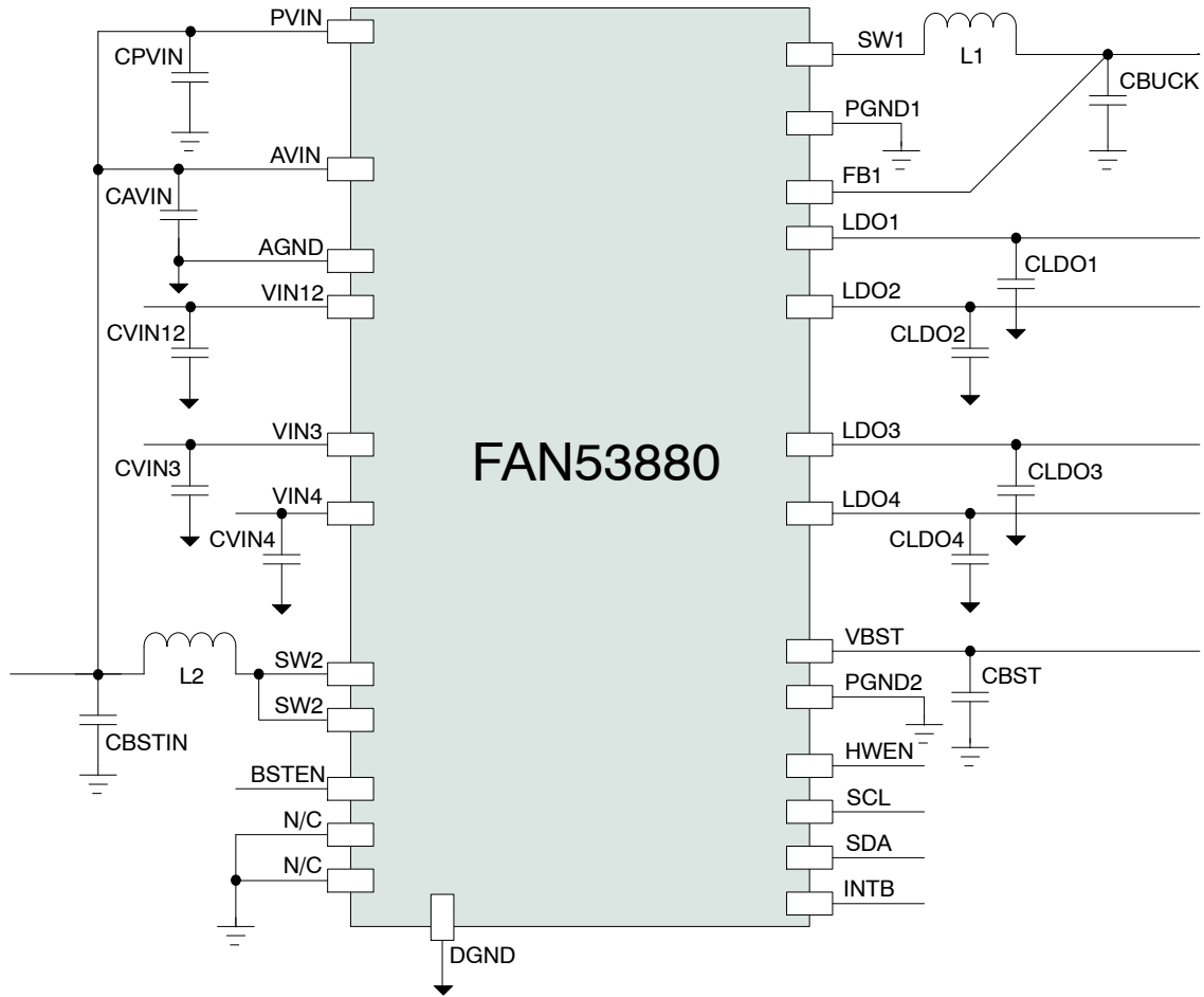
Figure 37. Application Diagram
