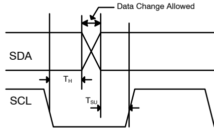
Figure 35. Data Transfer Timing
