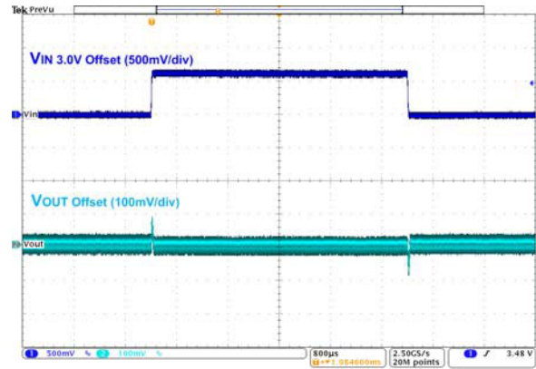
Figure 23. Line Transient, 3.0 \leftrightarrow 3.6 VIN, 10 ms Edge, 1500 mA Load, PWM
