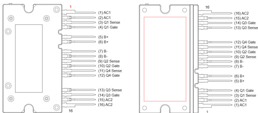
Figure 1. Pin Configuration
