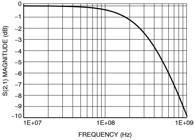
Figure 9. Insertion Loss
