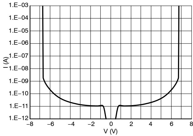
Figure 1. IV Characteristics
