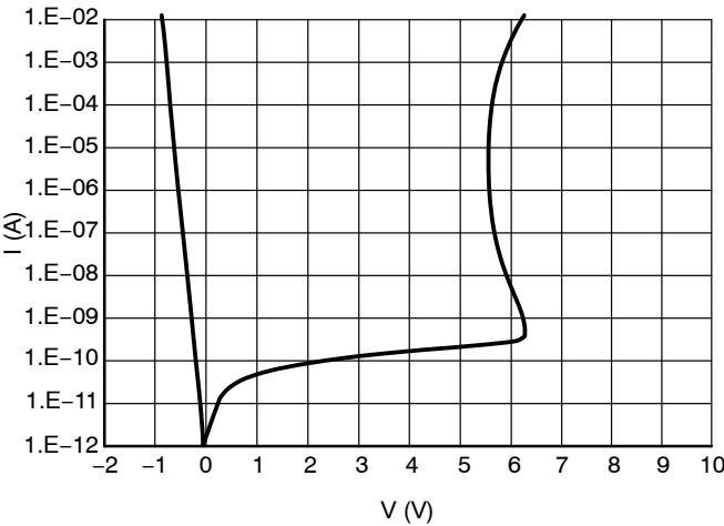
Figure 1. IV Characteristics
