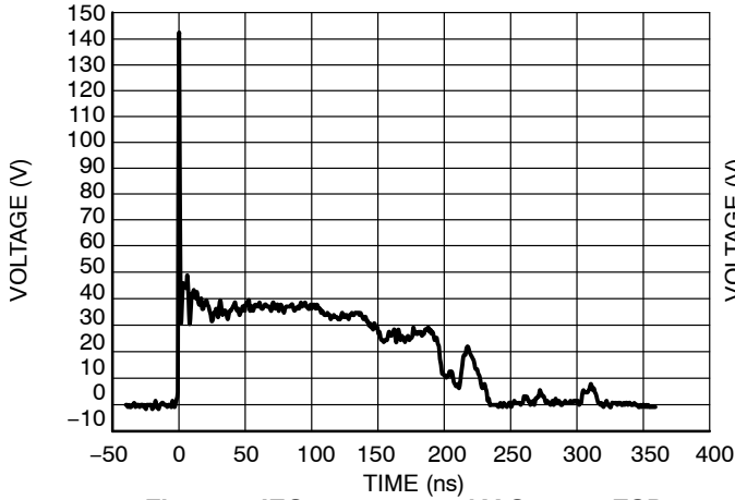
Figure 7. IEC61000-4-2 +8 kV Contact ESD Clamping Voltage
