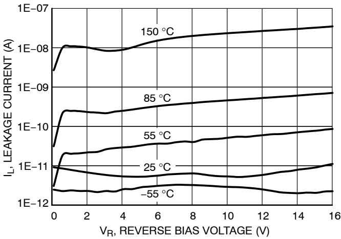
Figure 3. I_R vs. Temperature
