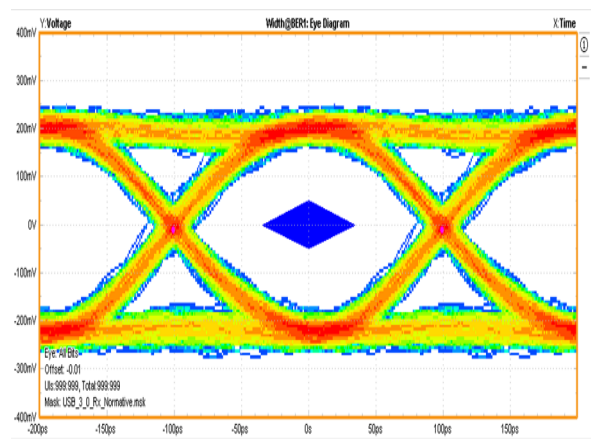
With ESD7002
