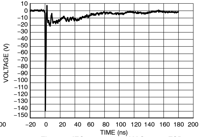
Figure 8. IEC61000-4-2 -8 kV Contact ESD Clamping Voltage
