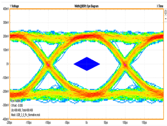
Without ESD7002
