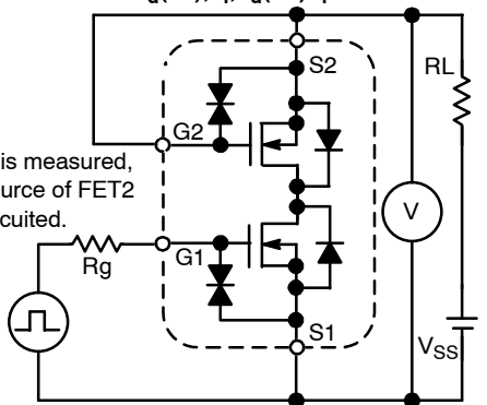
Test Circuit 7
