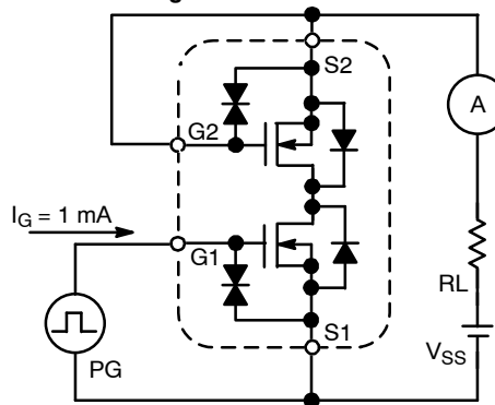
Test Circuit 6
