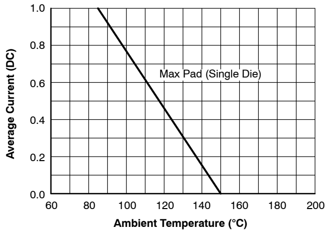
Figure 5. Maximum Average Current vs. Ambient Temperature
