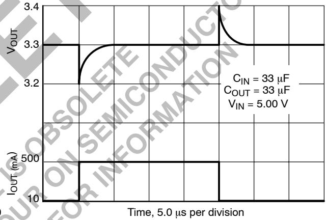
Figure 11. Transient Response
