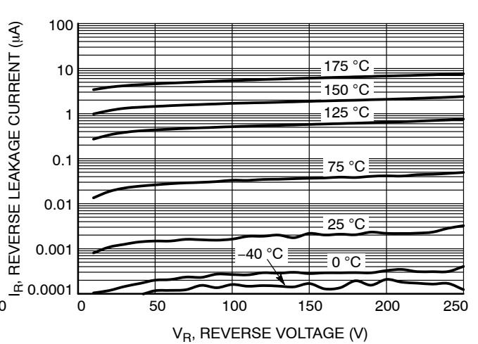
Figure 7. Reverse Current-BASH21
