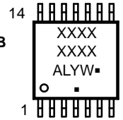
TSSOP-14 WB DT SUFFIX CASE 948G
