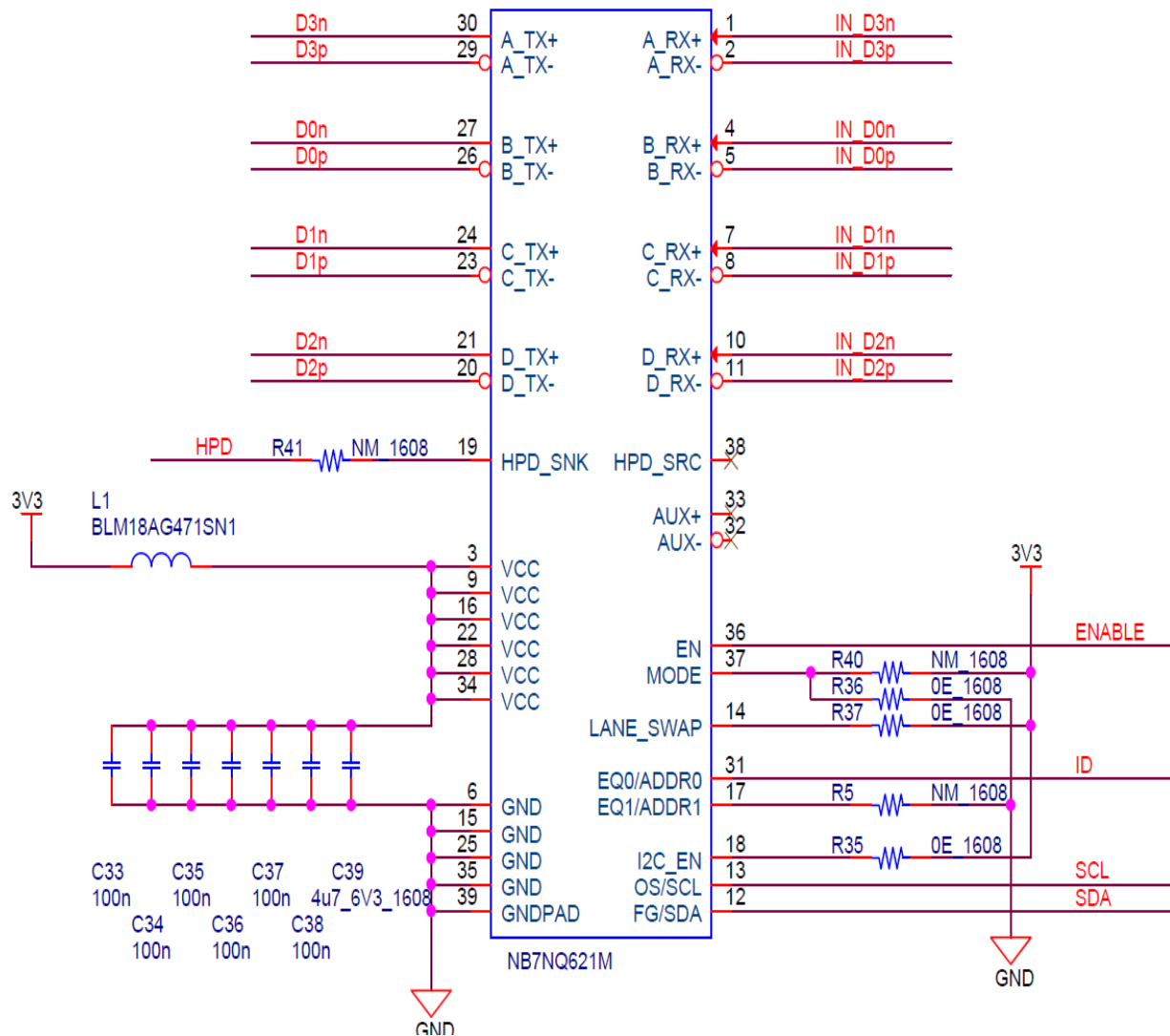
Figure 3. Sink Side Circuit
