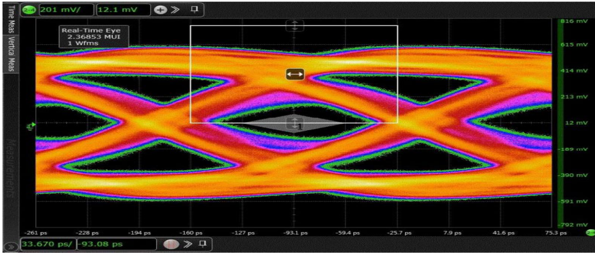
Figure 6. Eye-Diagram for HDMI 1.4 HF 7 – 10
