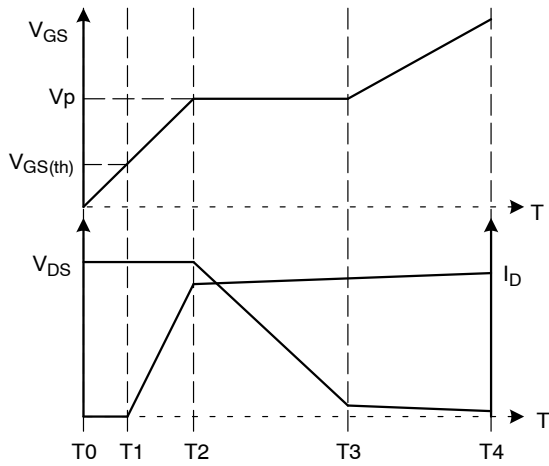
Figure 16. Gate Charge Waveforms
