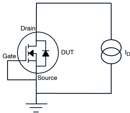
Figure 1. Drain-to-Source Breakdown Voltage Test Circuit
