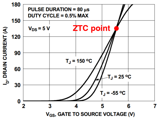
Figure 9. Transfer Characteristics
