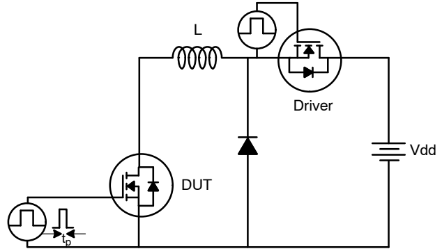
Figure 12. Unclamped Inductive Switching Test Circuit
