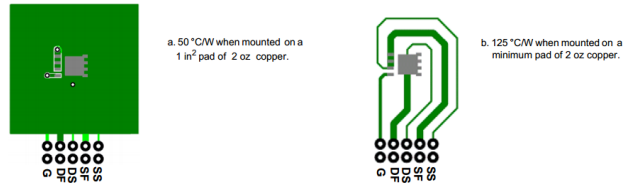
Figure 5. Mounted PCB Information for Thermal Resistance
