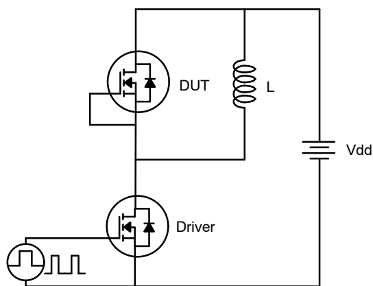
Figure 22. Reverse-Recovery Test Circuit
