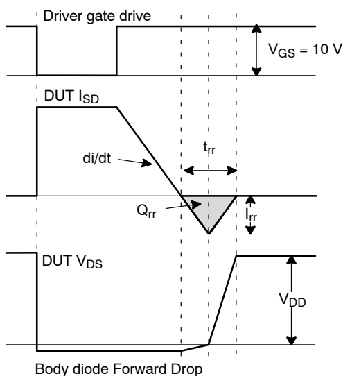
Figure 23. Reverse-Recovery Test Waveforms
