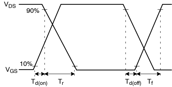
Figure 20. Switching Waveforms
