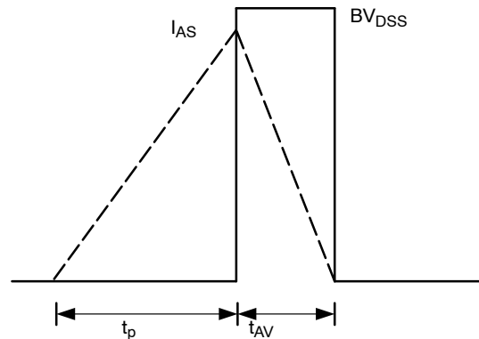
Figure 13. Unclamped Inductive Switching Waveforms
