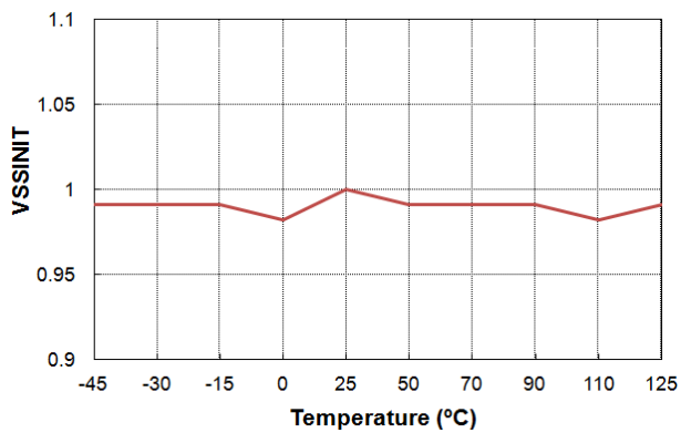
Figure 34. VSS.INIT vs. Temperature
