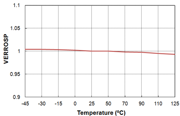
Figure 38. VERR.OSP vs. Temperature
