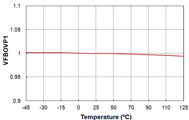
Figure 36. VFB.OVP1 vs. Temperature
