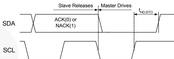
Figure 7. STOP Bit
